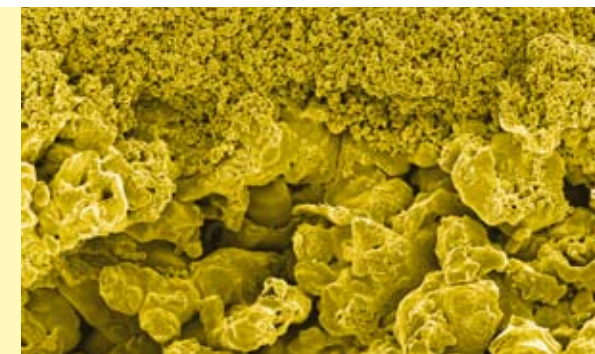
CO 2 splitting
