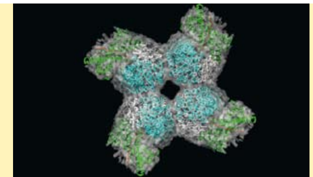
Photosynthesis In nature's power station
