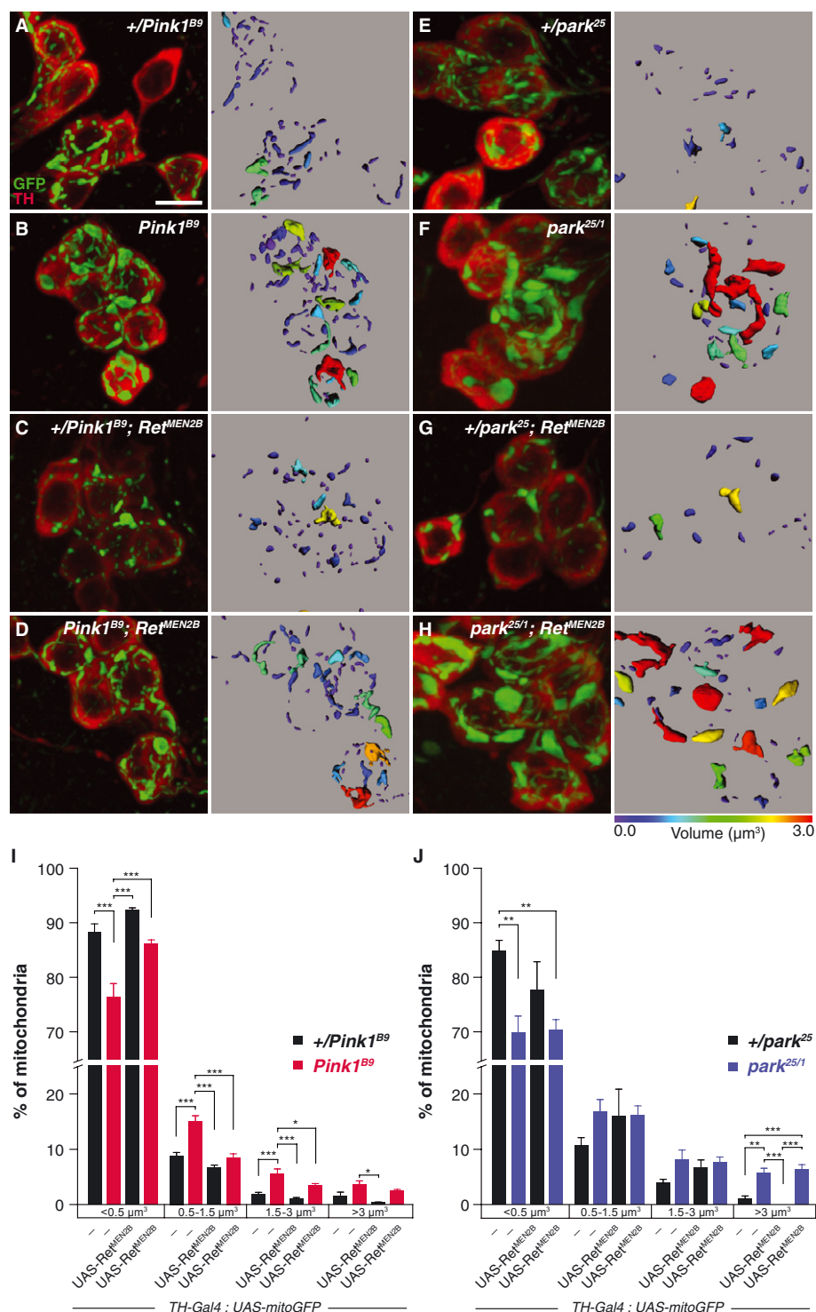
Figure 3. Rescue of Pink1 mutant dopamine neuron mitochondria by Ret MEN2B .
