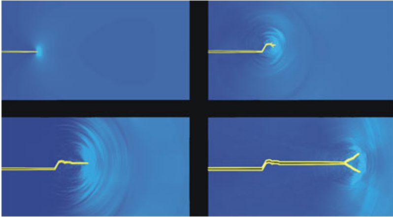
Image 2: Onset of fracture instabilities. At a critical crack speed, straight crack motion becomes unstable and the crack starts to wiggle, creating increasingly rough fracture surfaces.
